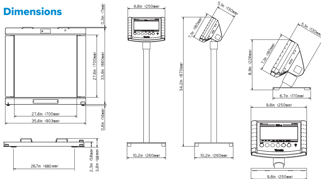
Tall and short pillar indicator options available
